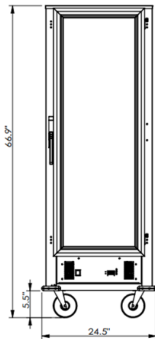
Front View
